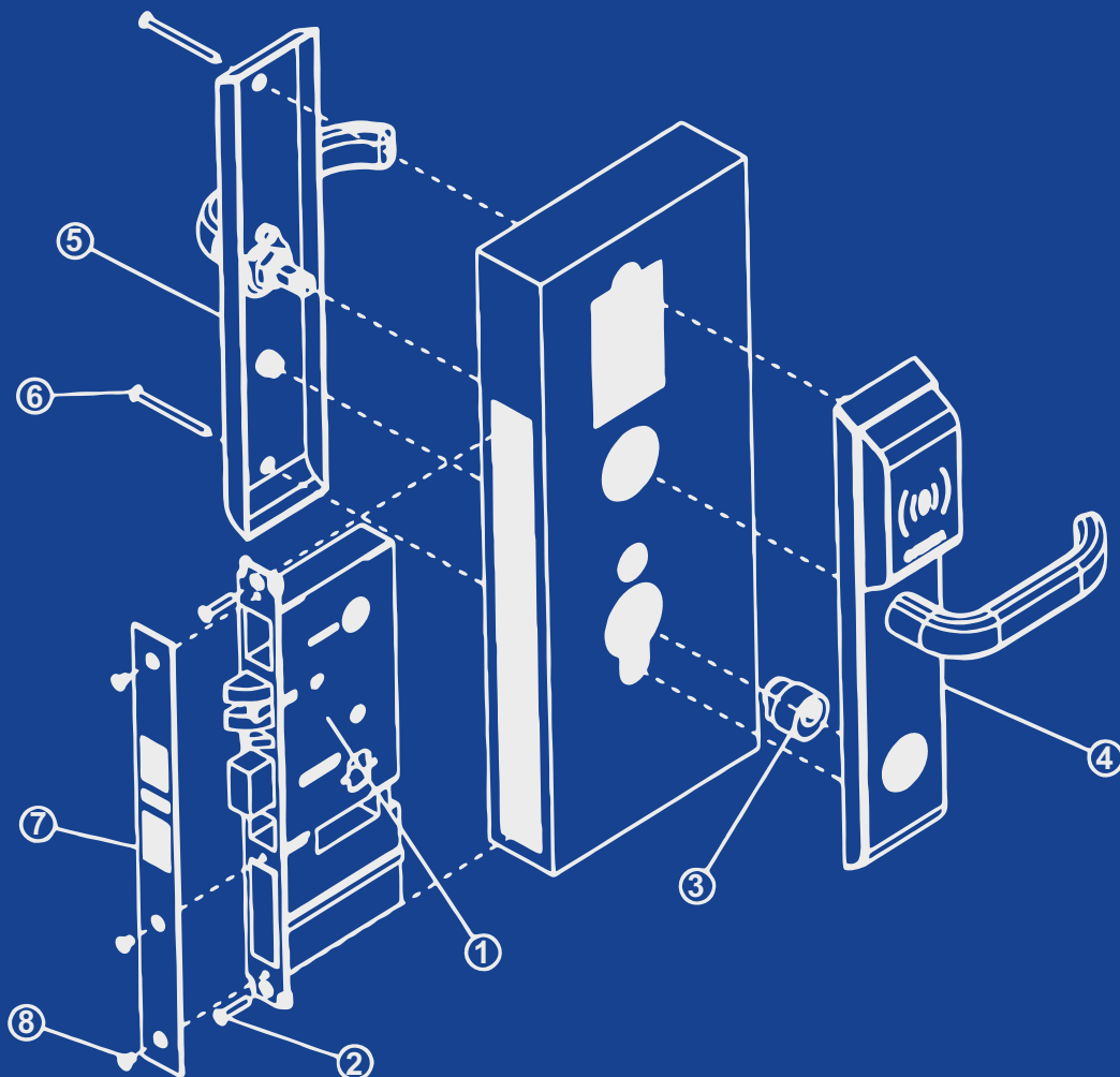
Installation Diagram
